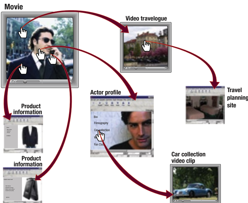
Figure 4: Video Browsing
